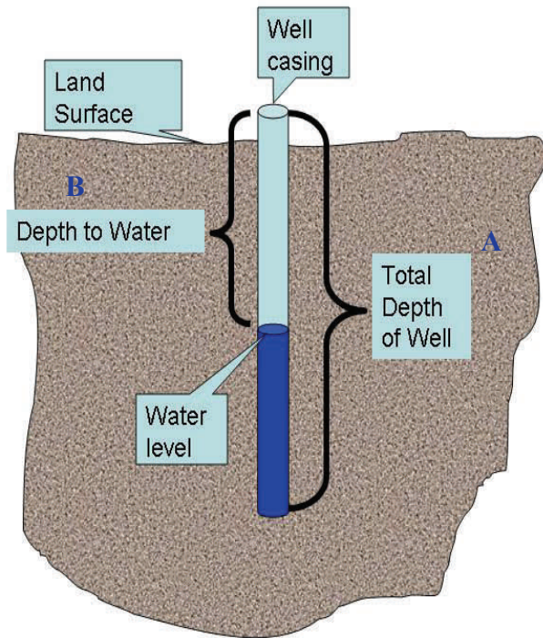
Figure 1: Use a clean tape measure or a string to estimate the depth of standing water in a well. The depth of standing water is the difference between the total depth (A) and the depth to water (B).
